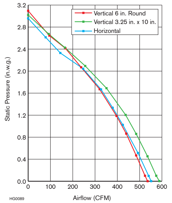
Airflow Performance at High Speed
