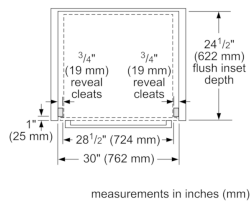
Standard installation Single oven, double oven or combo oven over warming or storage drawer
