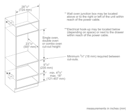
Flush installation Double or combo oven over storage or warming drawer
