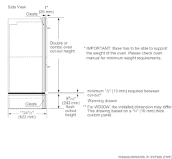
Side View-Combination Oven with Microwave or Speed Oven
